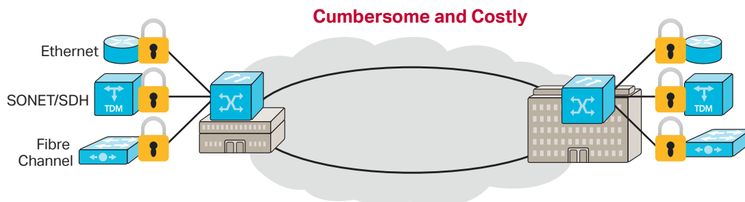
Figure 2. Traditional, protocol-specific encryption deployed in a multiservice network
